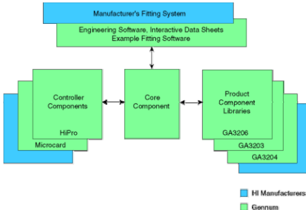
Figure 1: An overview of the ARK components and applications
